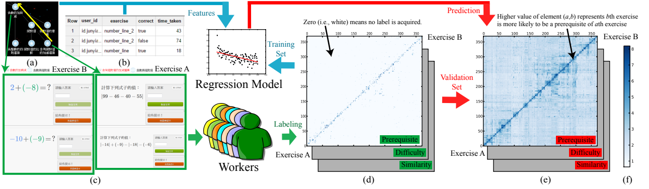
Figure 2: The proposed work flow. (a) A screen shot of the local knowledge map, (b) examples of usage log, (c) a example of exercise pairs, (d) the sparse similarity matrices labeled by workers, (e) the dense similarity matrices predicted by a regression model, and (f) the color code of (d) and (e).
